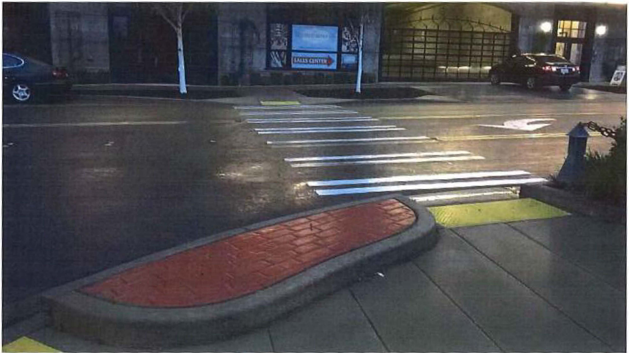
Example of Broadway LID project improvements
